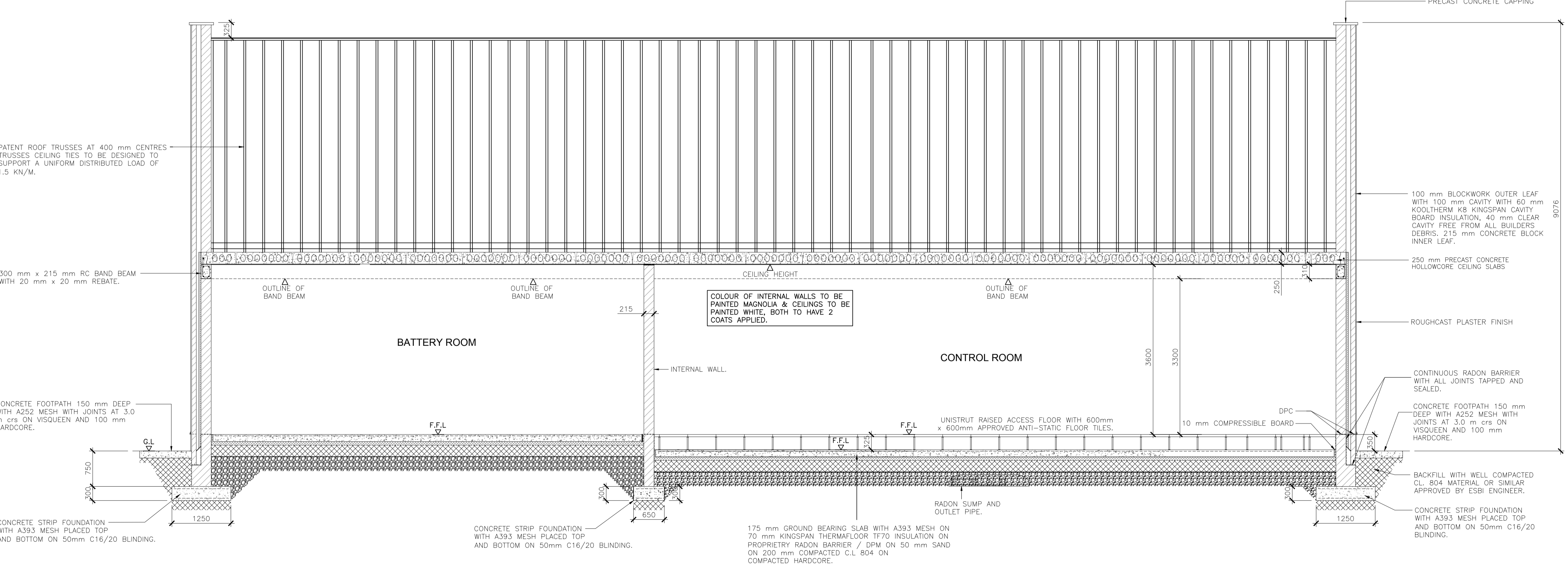
SECTION B SCALE 1:50
